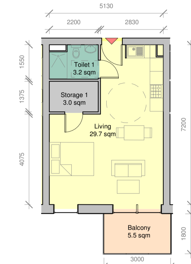
Proposed Studio Apartment - Type 5B Scale 1:100
