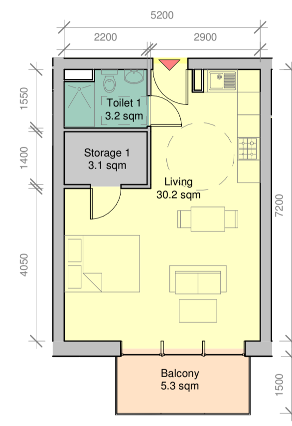
Proposed Studio Apartment - Type 5A Scale 1:100
