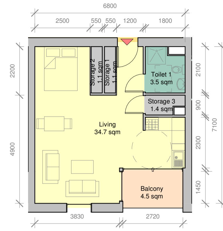
Proposed Studio Apartment - Type 2 Scale 1:100
