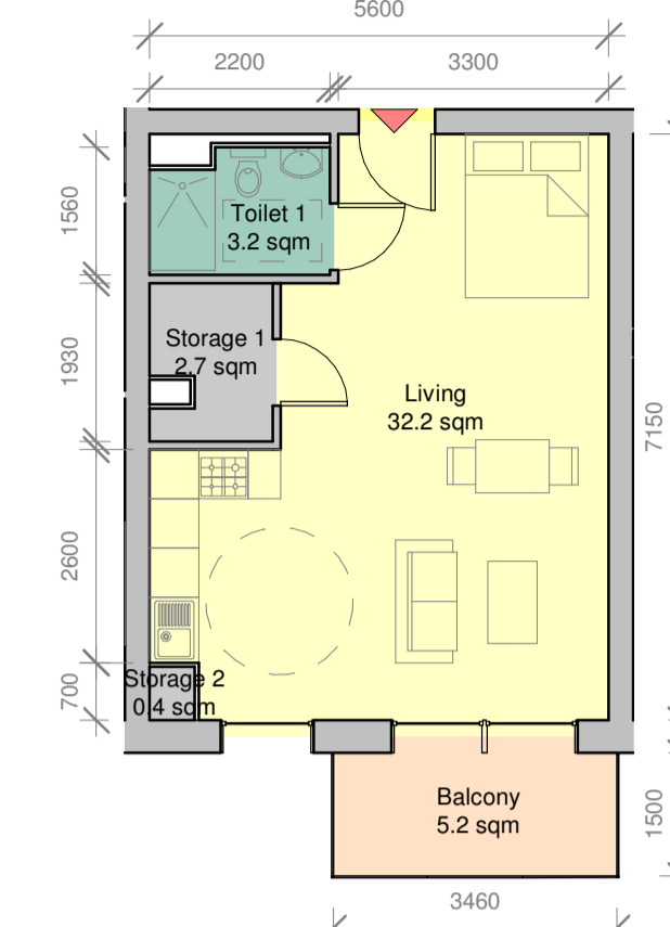
Proposed Studio Apartment - Type 3B Scale 1:100
