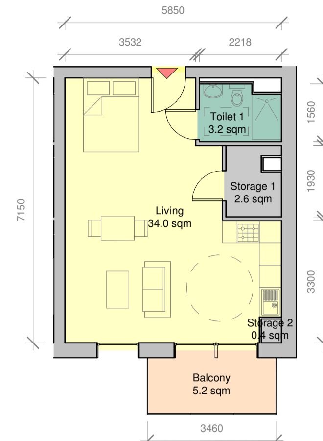
Proposed Studio Apartment - Type 3A Scale 1:100
