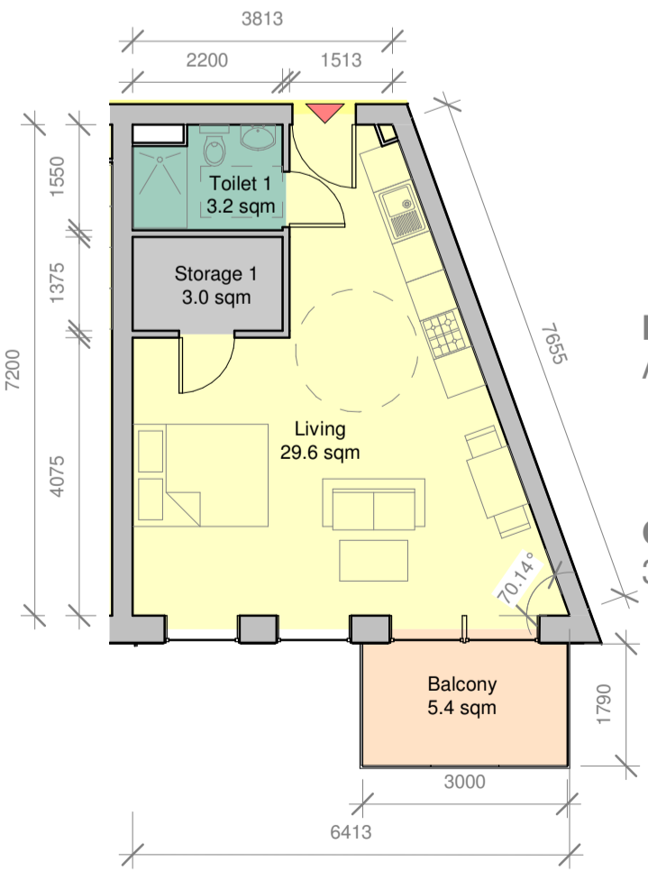
Proposed Studio Apartment - Type 6 Scale 1:100
