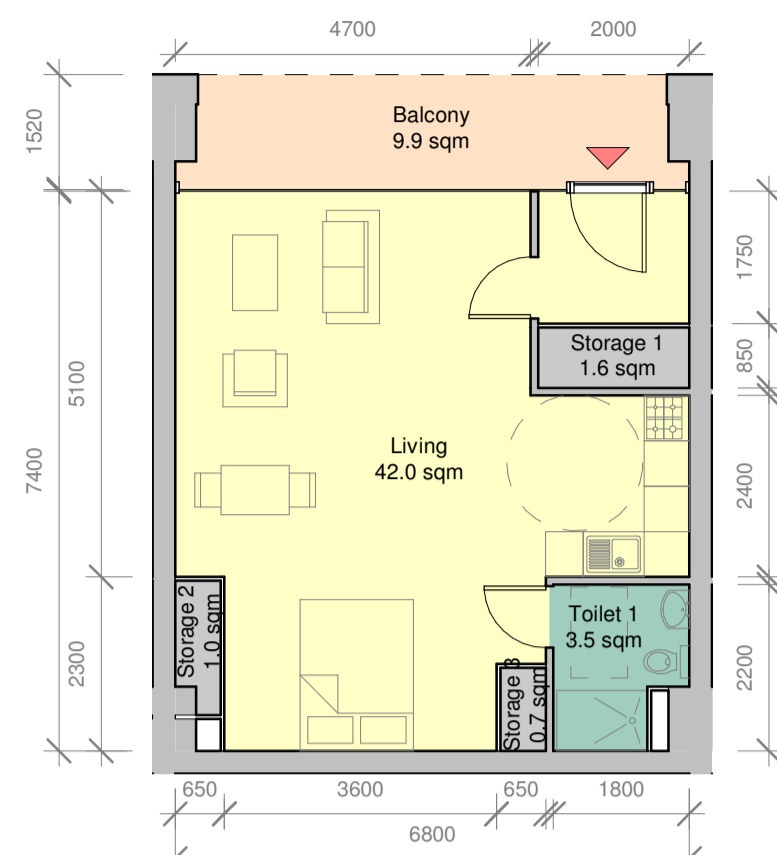
Proposed Studio Apartment - Type 1 Scale 1:100
