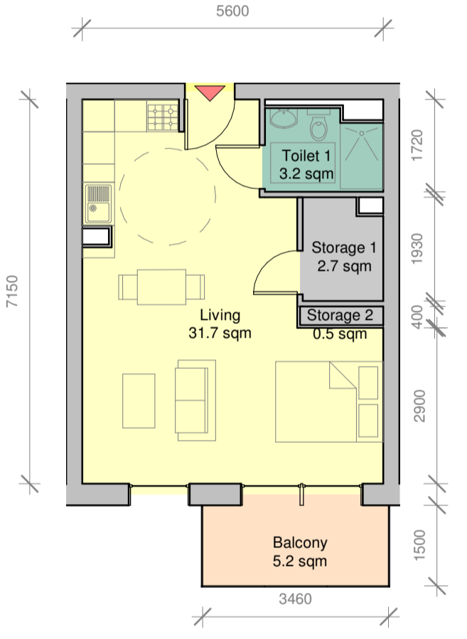
Proposed Studio Apartment - Type 4 Scale 1:100
