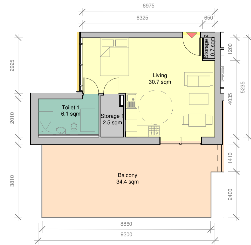
Proposed Studio Apartment - Type 7 Scale 1:100
