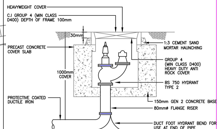
TYPICAL INDICATIVE FIRE HYDRANT NOT TO SCALE
