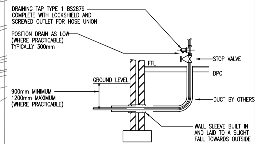
INCOMING MWS ENTRY DETAIL NOT TO SCALE
